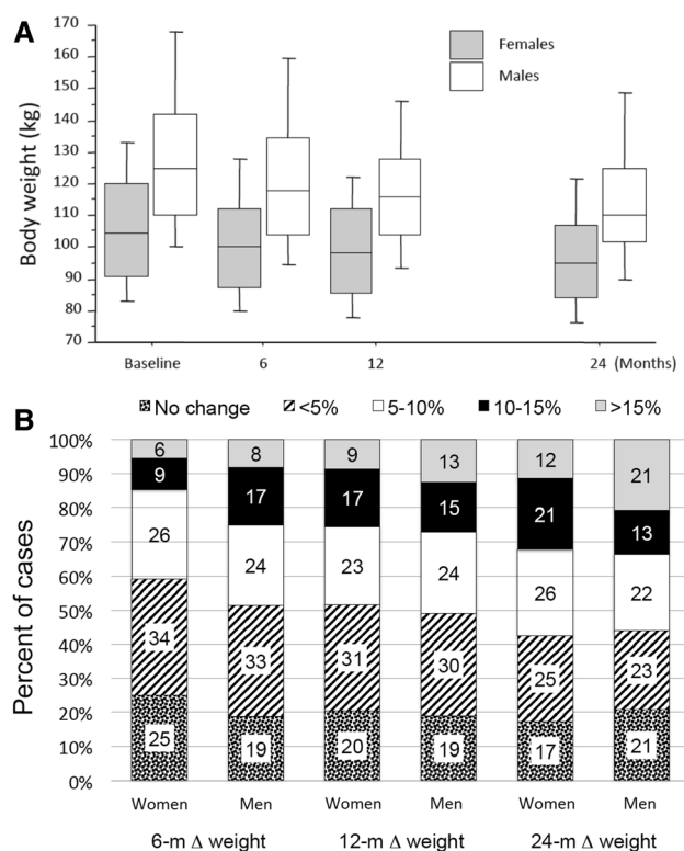
Fig. 1 a Time course of body weight in subjects compliant to follow-up (upper panel). b Percent of cases attaining short- and long-term weight loss targets in relation to gender (lower panel). Panel A: the box indicates the area of 25°–75° percentiles (and median); the whiskers stretch to 5° and 95° percentile. Panel B: the numbers inside the columns are the percentage of cases, in relation to weight loss targets
